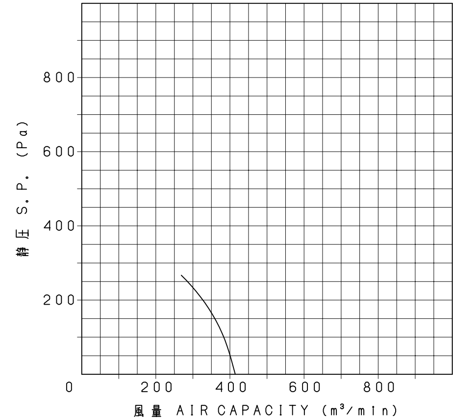
特性曲線 CHARACTERISTIC CURVE JIS B8330 (at+20°C)
