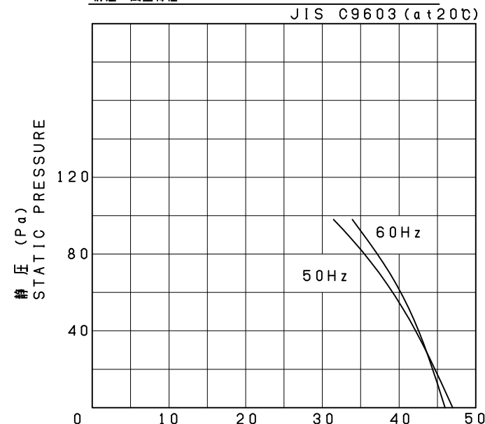
静圧・風量特性 CHARACTERISTICS CURVE
