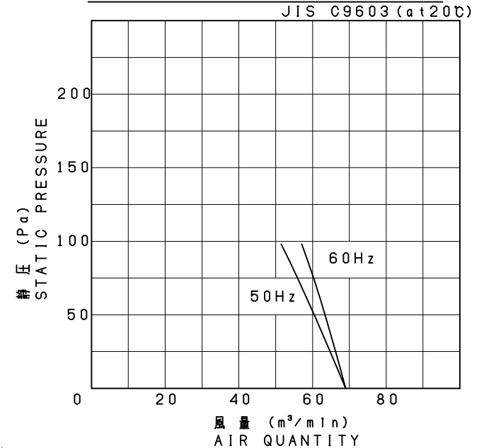
静圧・風量特性 CHARACTERISTICS CURVE
