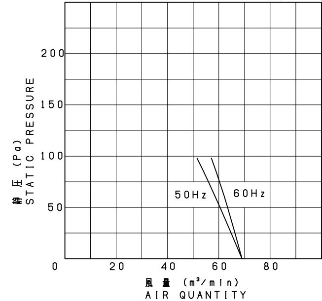
静圧・風量特性 CHARACTERISTICS CURVE
