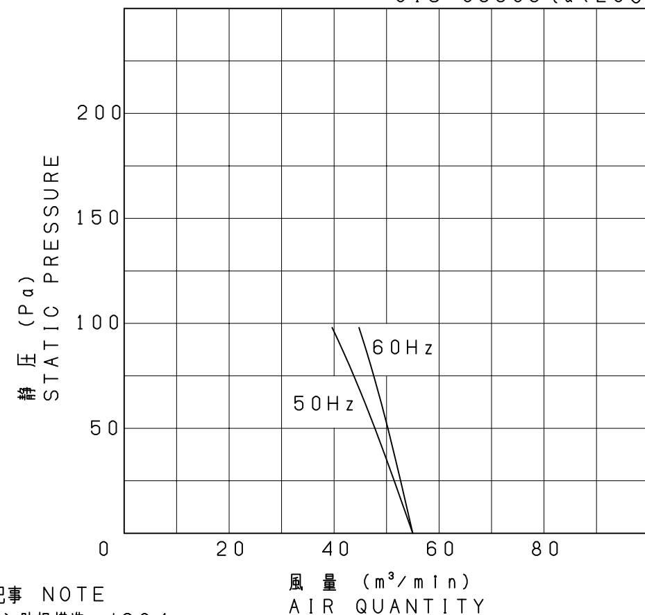
静圧・風量特性 CHARACTERISTICS CURVE JIS C9603 (at 20℃)
