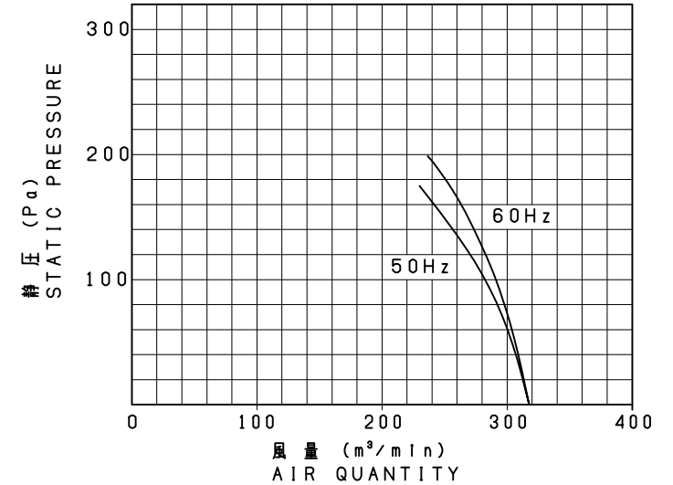
静圧・風量特性 CHARACTERISTICS CURVE JIS B8330 (at 20℃)
